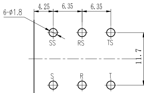
PCB Layout (TOP VIEW) Tolerance: \pm 0.05
