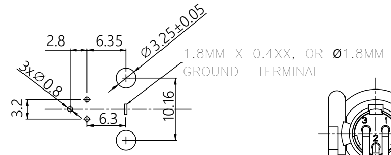
PCB Footprint (Top Side)
