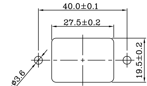
PANEL CUT-OUT
